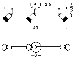
Base 660007 Copper Metal GU10 3x50 Watt 230 Volt IP20 Bulb Excluded L: 49 W:8 H: 10.9 cm
