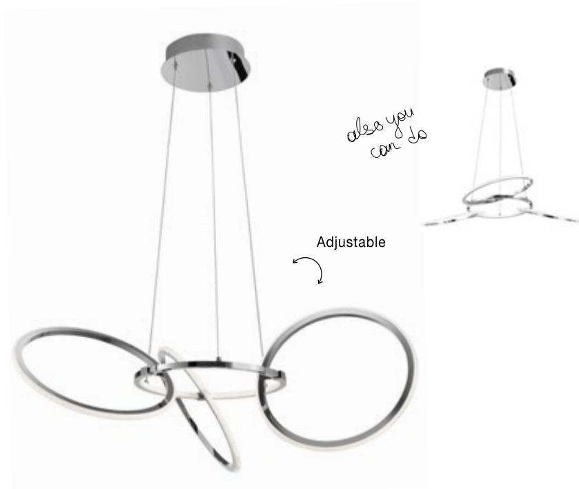
Dante 9008011 Chrome Aluminium & Acrylic Adjustable LED 39 Watt 230 Volt 1900Lm 3000K IP20 D: 70 H: 150 cm LED WARM WHITE A+++ DRIVER INCL.
