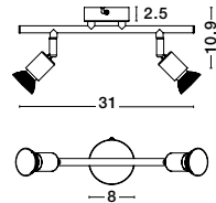
Base 660006 Copper Metal GU10 2x50 Watt 230 Volt IP20 Bulb Excluded L: 31 W:8 H: 10.9 cm
